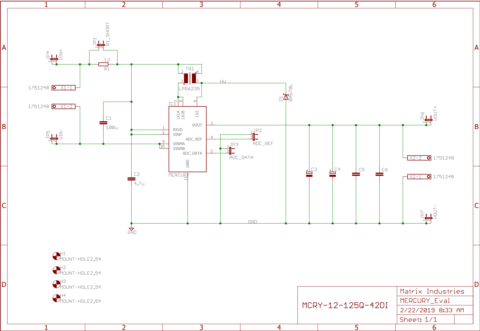
Figure 4: MCEY-EVALKIT Schematics
